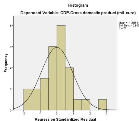
Figure 4. Histogram
